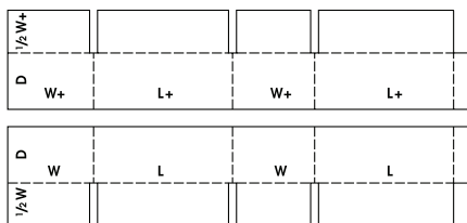
0320 Full Telescope Half Slotted Container (FTHS)
