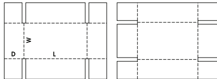
0301 Full Telescope Design Style Container (FTD)
